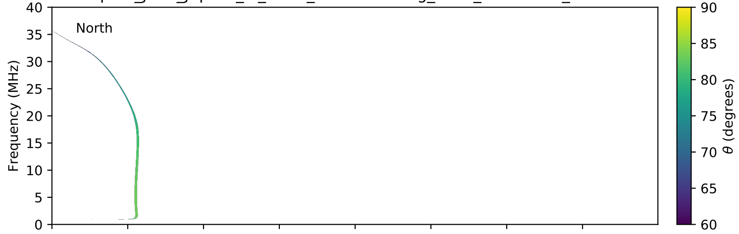
expres_juno_jupiter_io_isaac_lossc-wid1deg_3kev_20160106_v01.cdf
