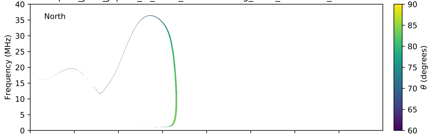
expres_juno_jupiter_io_isaac_lossc-wid1deg_3kev_20160104_v01.cdf
