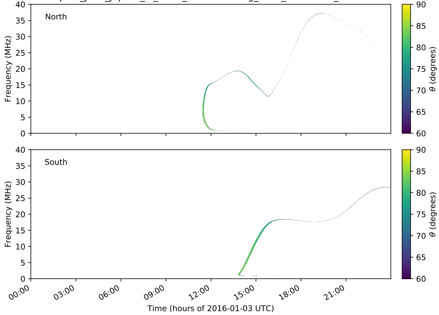
expres_juno_jupiter_io_isaac_lossc-wid1deg_3kev_20160103_v01.cdf
