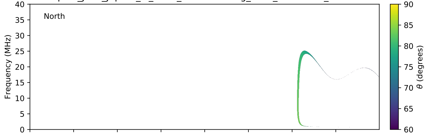
expres_juno_jupiter_io_isaac_lossc-wid1deg_3kev_20160101_v01.cdf
