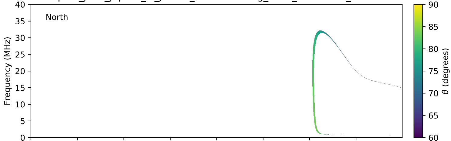
expres_juno_jupiter_io_JRM09_lossc-wid1deg_3kev_20160101_v01.cdf
