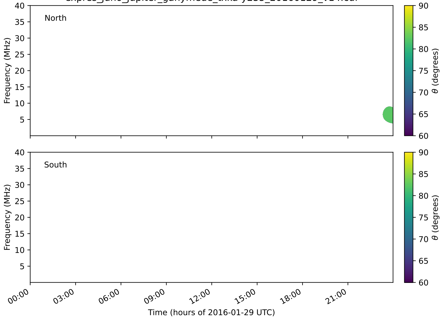
expres_juno_jupiter_ganymede_txka-y235_20160129_v14.cdf
