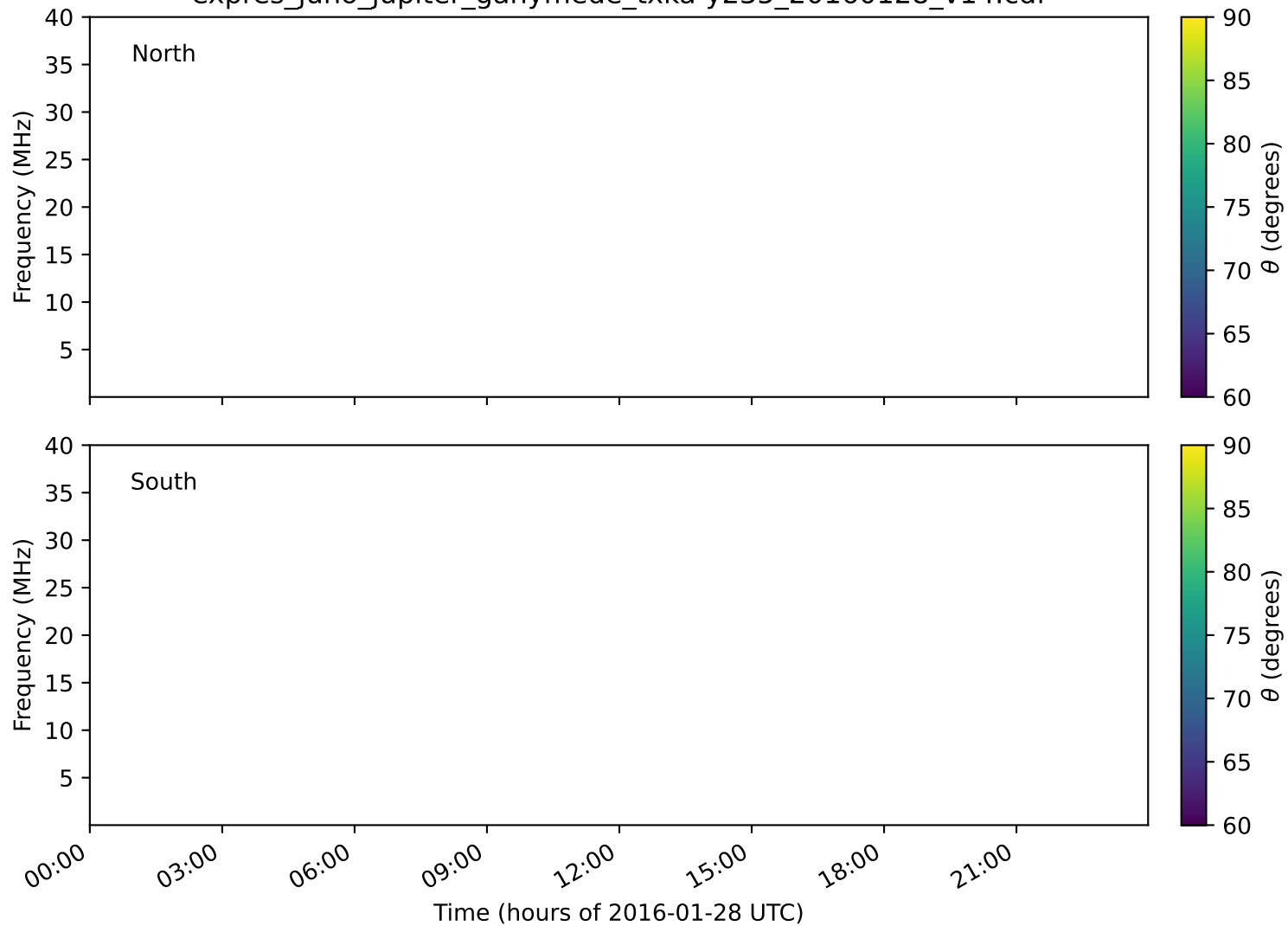
expres_juno_jupiter_ganymede_txka-y235_20160128_v14.cdf
