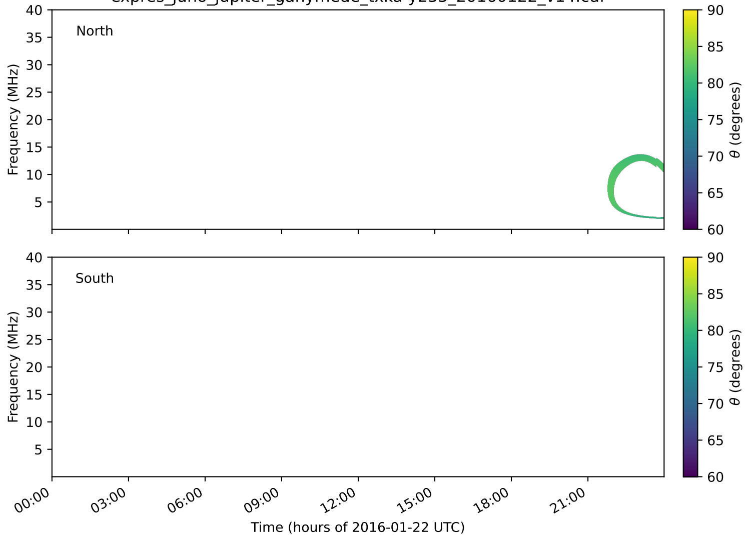
expres_juno_jupiter_ganymede_txka-y235_20160122_v14.cdf
