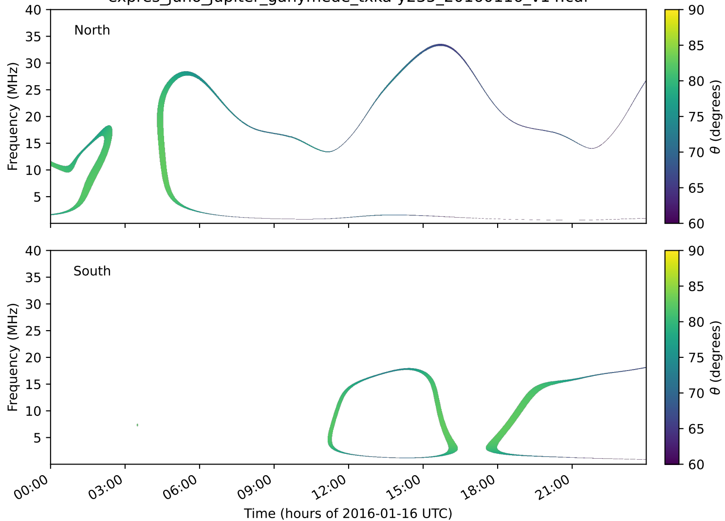
expres_juno_jupiter_ganymede_txka-y235_20160116_v14.cdf
