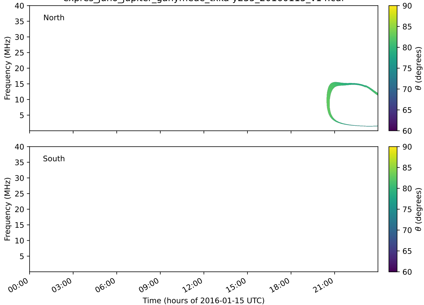
expres_juno_jupiter_ganymede_txka-y235_20160115_v14.cdf
