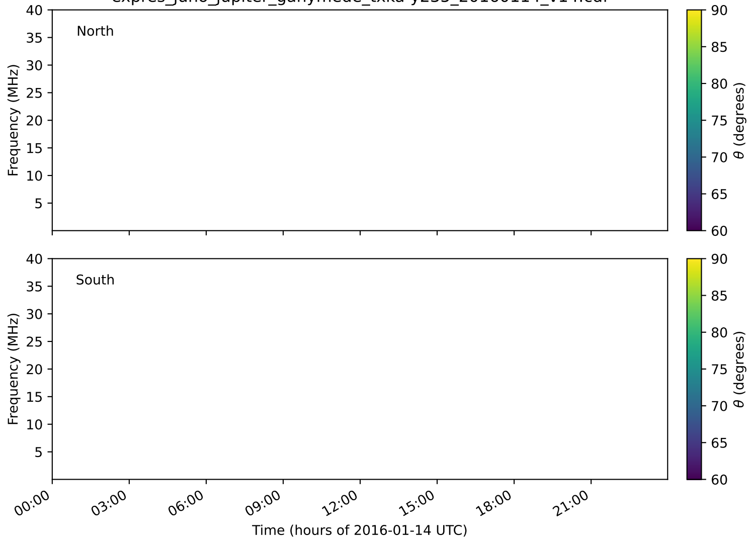
expres_juno_jupiter_ganymede_txka-y235_20160114_v14.cdf
