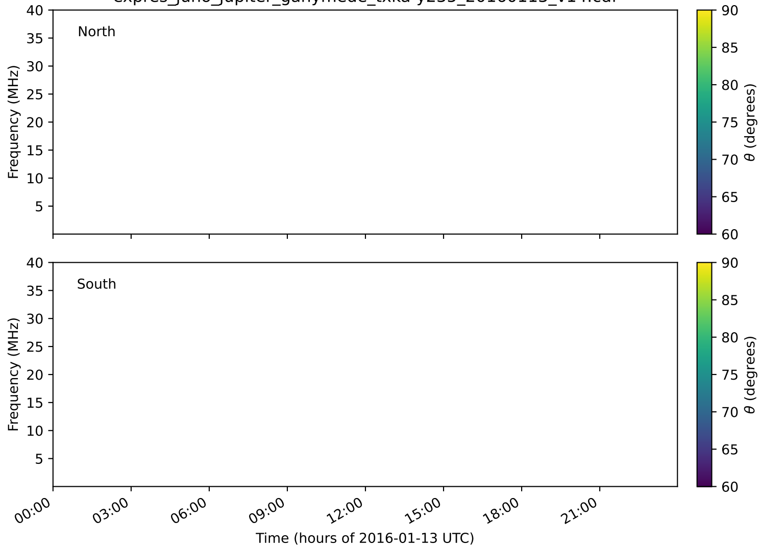
expres_juno_jupiter_ganymede_txka-y235_20160113_v14.cdf
