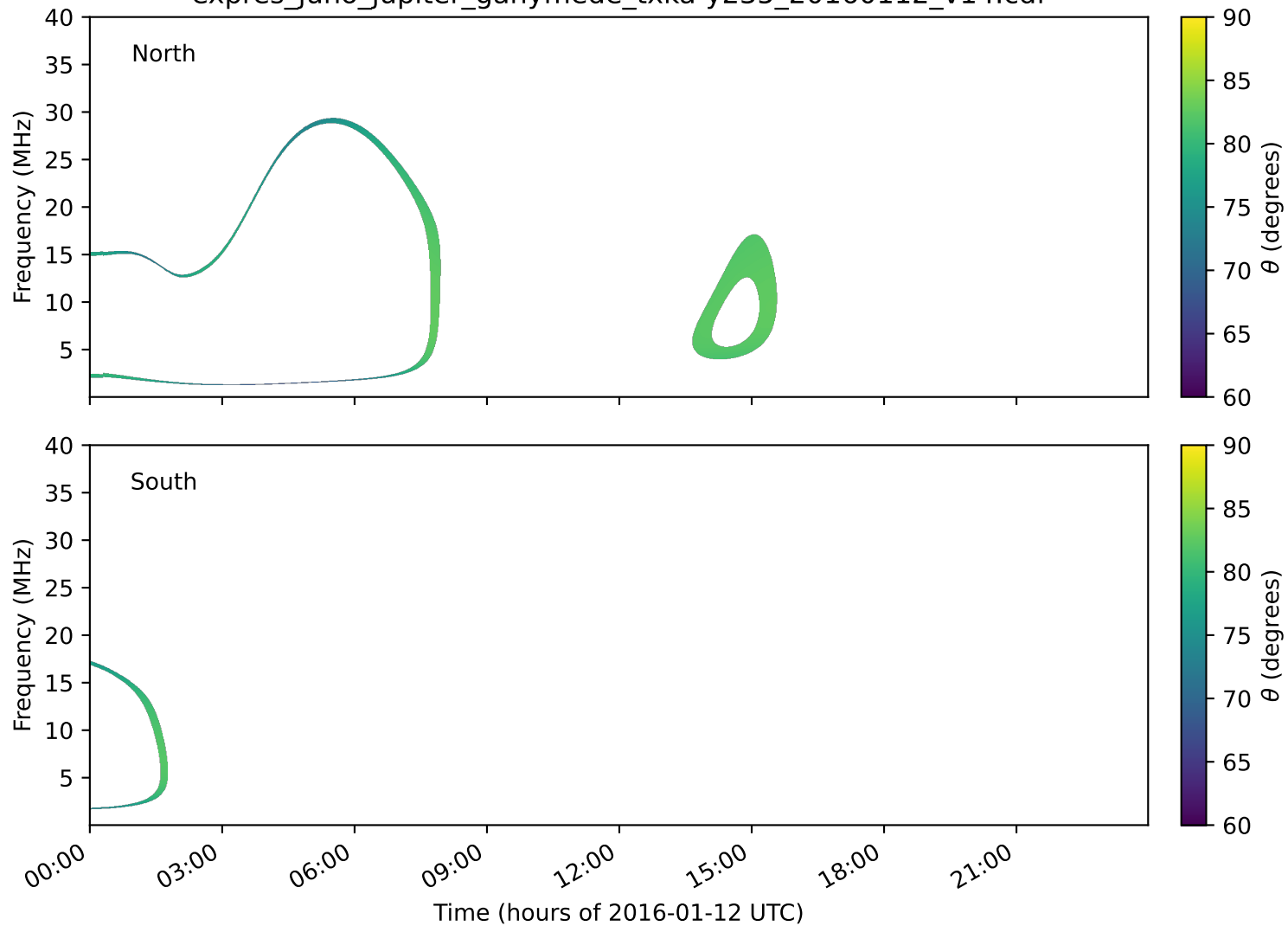
expres_juno_jupiter_ganymede_txka-y235_20160112_v14.cdf
