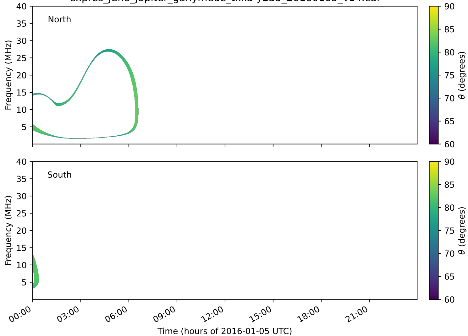
expres_juno_jupiter_ganymede_txka-y235_20160105_v14.cdf
