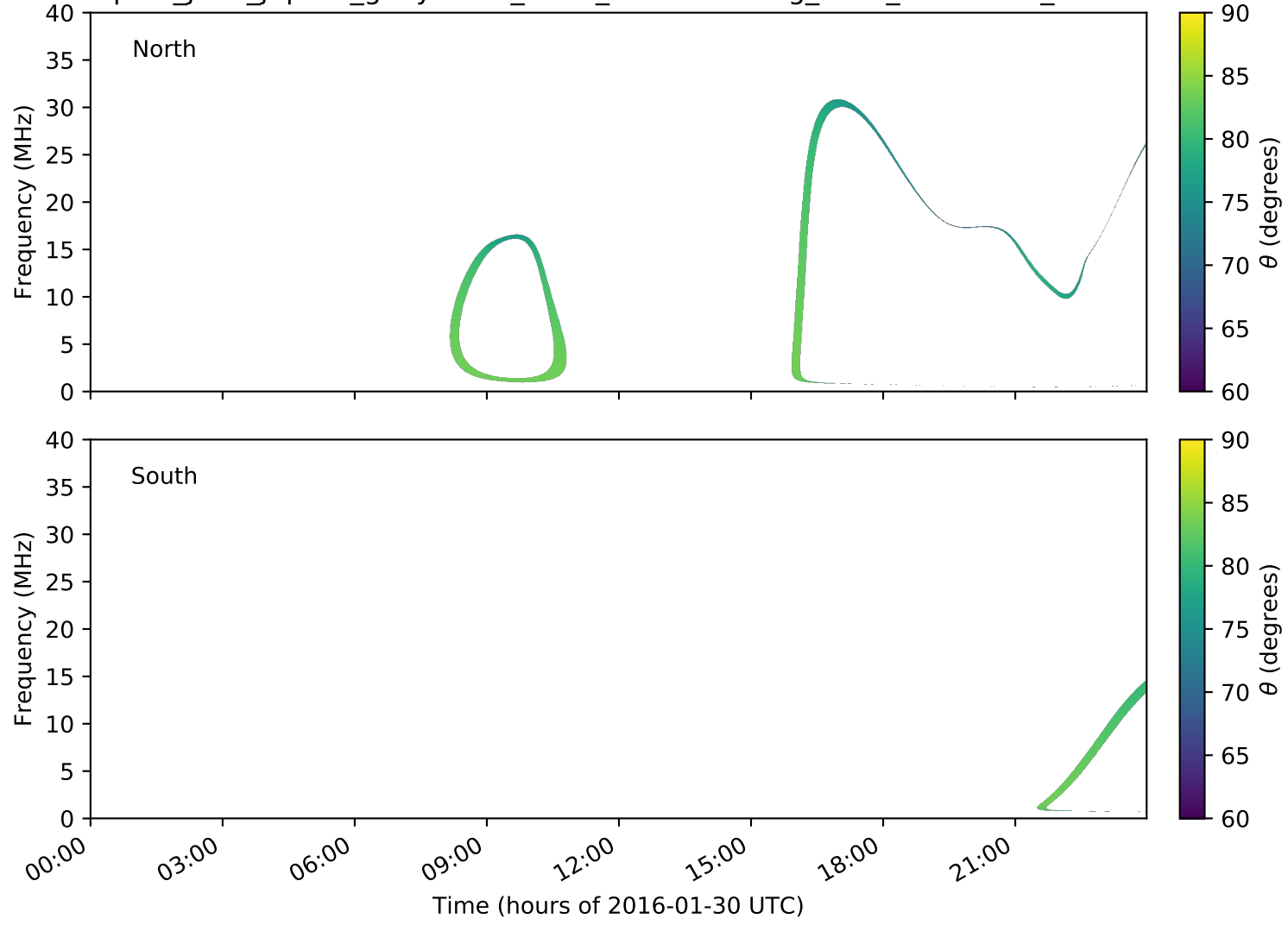
expres_juno_jupiter_ganymede_isaac_lossc-wid1deg_3kev_20160130_v01.cdf
