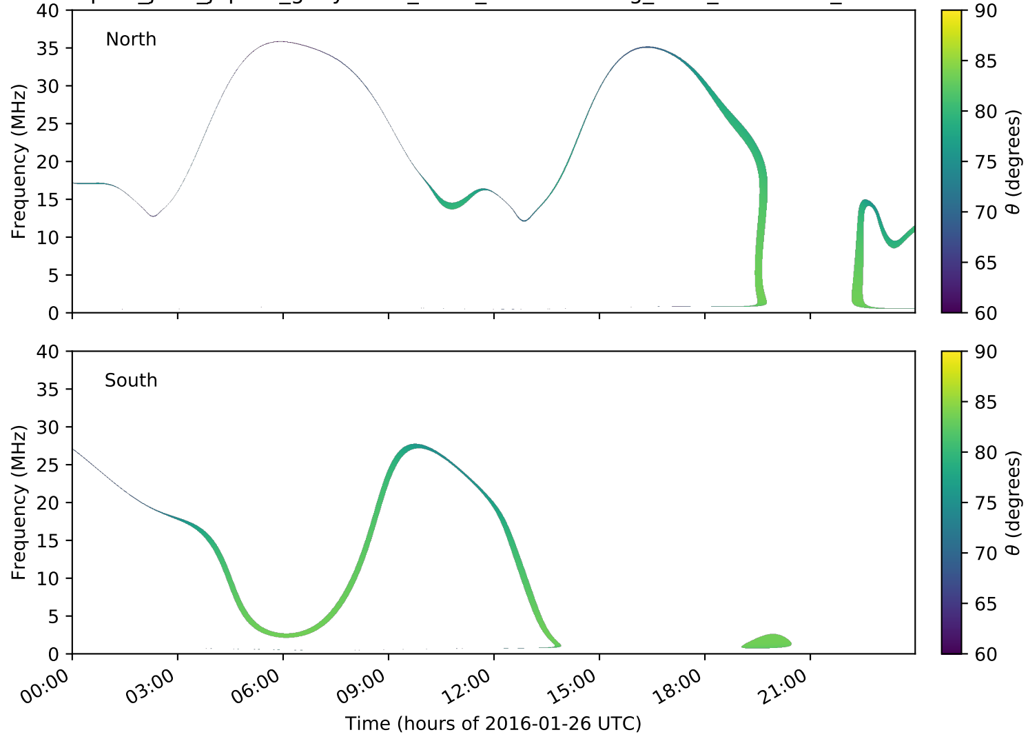
expres_juno_jupiter_ganymede_isaac_lossc-wid1deg_3kev_20160126_v01.cdf
