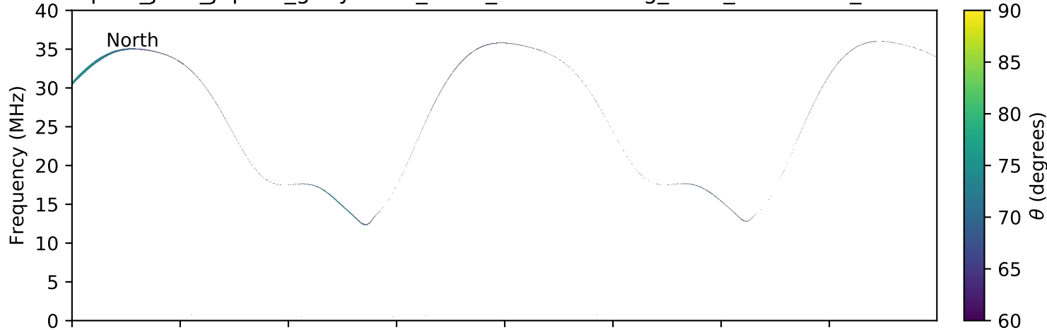
expres_juno_jupiter_ganymede_isaac_lossc-wid1deg_3kev_20160124_v01.cdf
