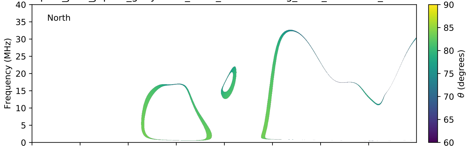
expres_juno_jupiter_ganymede_isaac_lossc-wid1deg_3kev_20160123_v01.cdf
