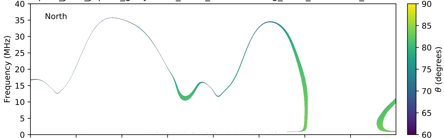
expres_juno_jupiter_ganymede_isaac_lossc-wid1deg_3kev_20160119_v01.cdf
