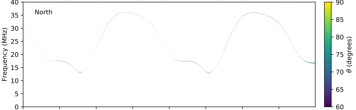
expres_juno_jupiter_ganymede_isaac_lossc-wid1deg_3kev_20160118_v01.cdf
