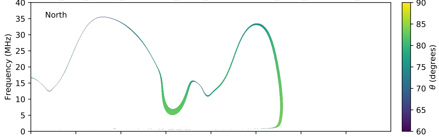
expres_juno_jupiter_ganymede_isaac_lossc-wid1deg_3kev_20160112_v01.cdf
