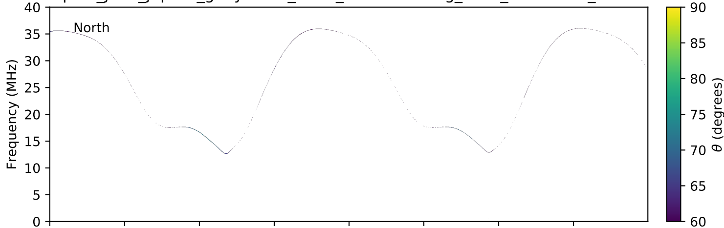
expres_juno_jupiter_ganymede_isaac_lossc-wid1deg_3kev_20160110_v01.cdf
