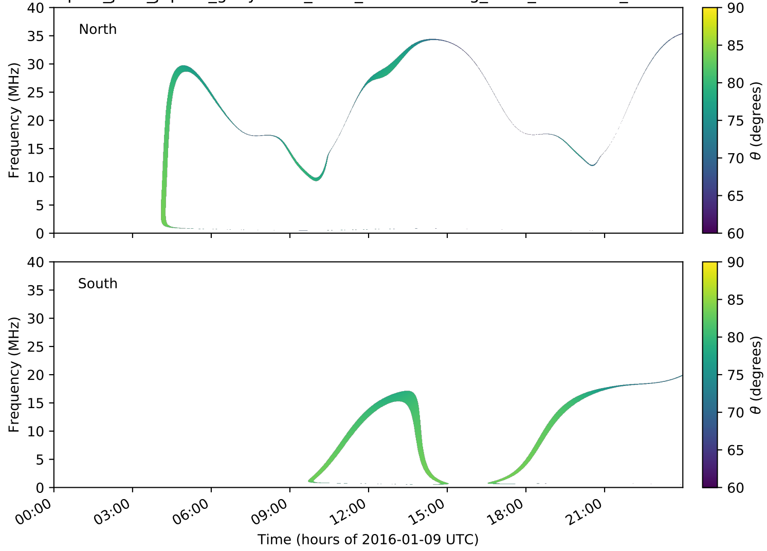
expres_juno_jupiter_ganymede_isaac_lossc-wid1deg_3kev_20160109_v01.cdf
