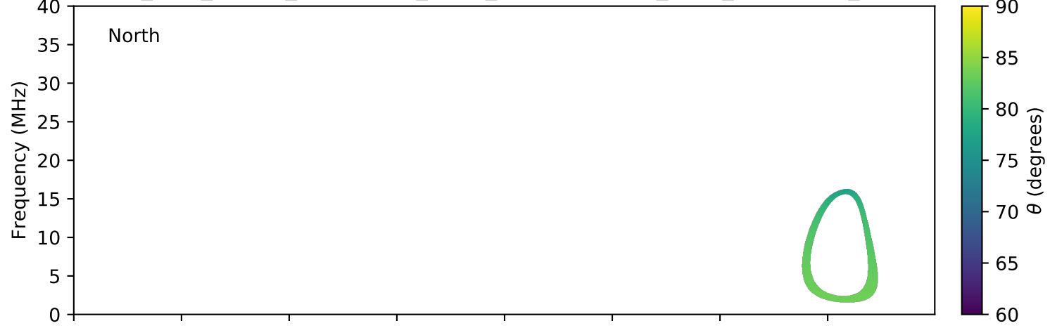
expres_juno_jupiter_ganymede_isaac_lossc-wid1deg_3kev_20160108_v01.cdf
