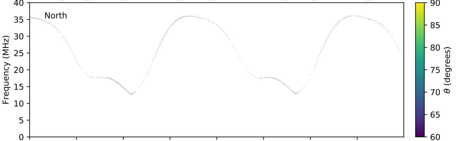
expres_juno_jupiter_ganymede_isaac_lossc-wid1deg_3kev_20160103_v01.cdf
