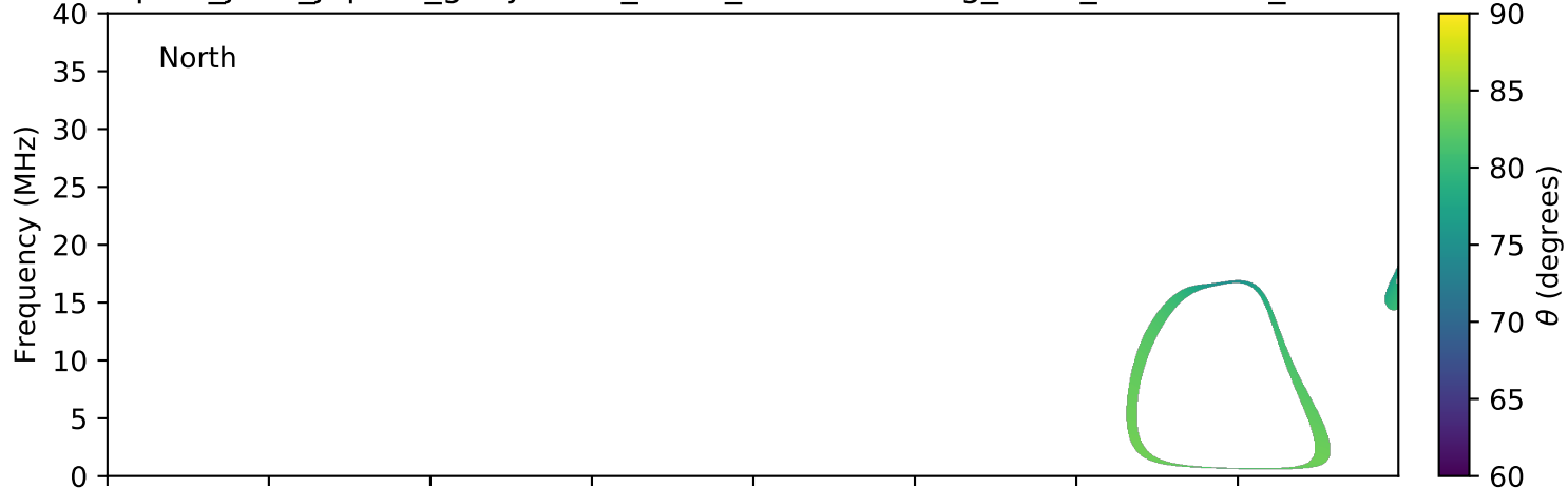
expres_juno_jupiter_ganymede_isaac_lossc-wid1deg_3kev_20160101_v01.cdf
