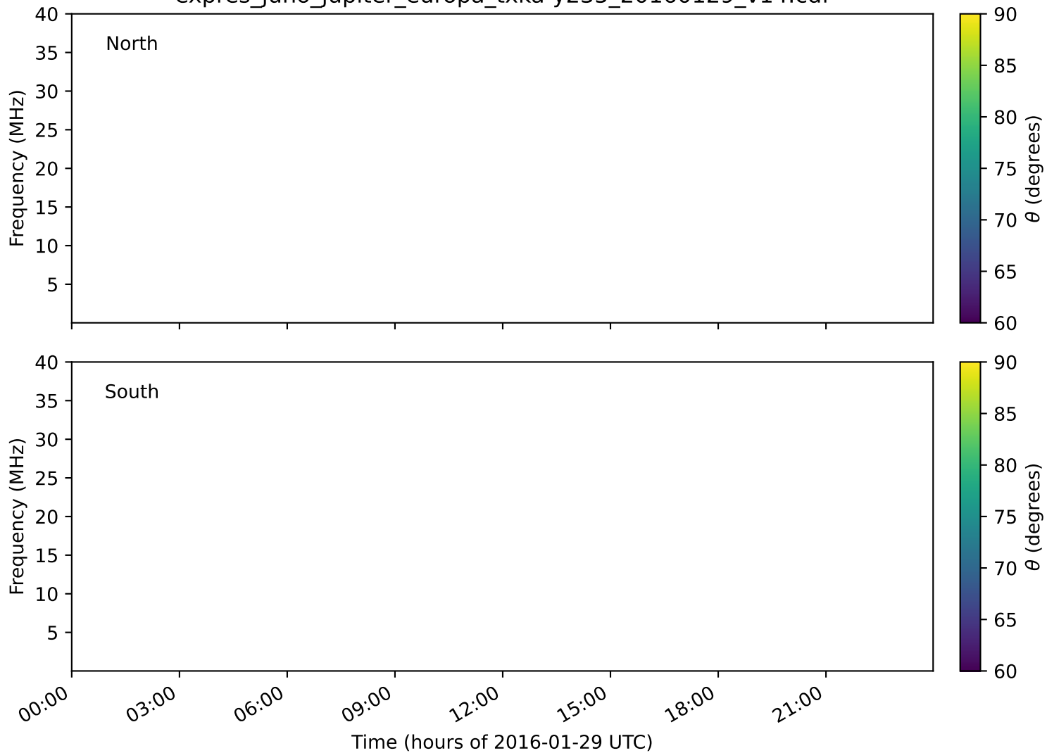
expres_juno_jupiter_europa_txka-y235_20160129_v14.cdf
