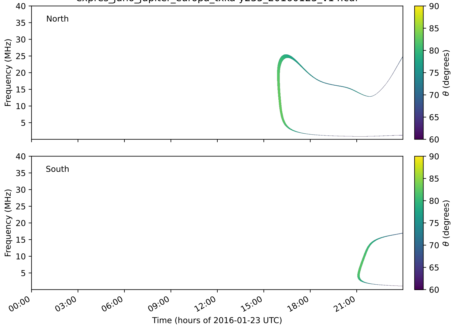
expres_juno_jupiter_europa_txka-y235_20160123_v14.cdf
