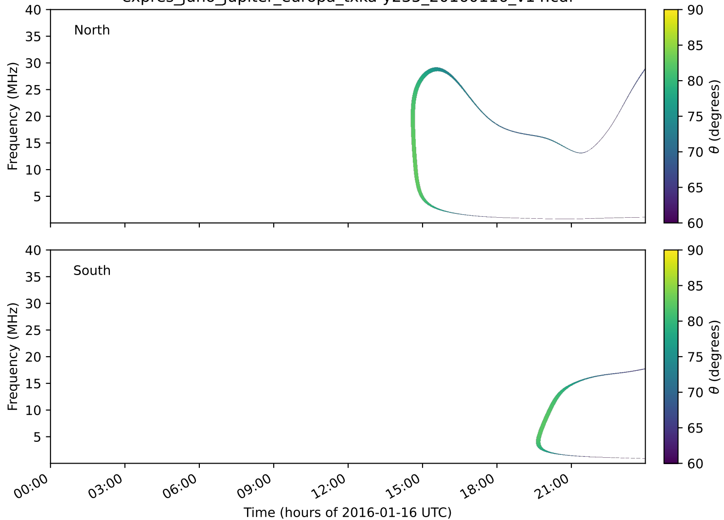
expres_juno_jupiter_europa_txka-y235_20160116_v14.cdf
