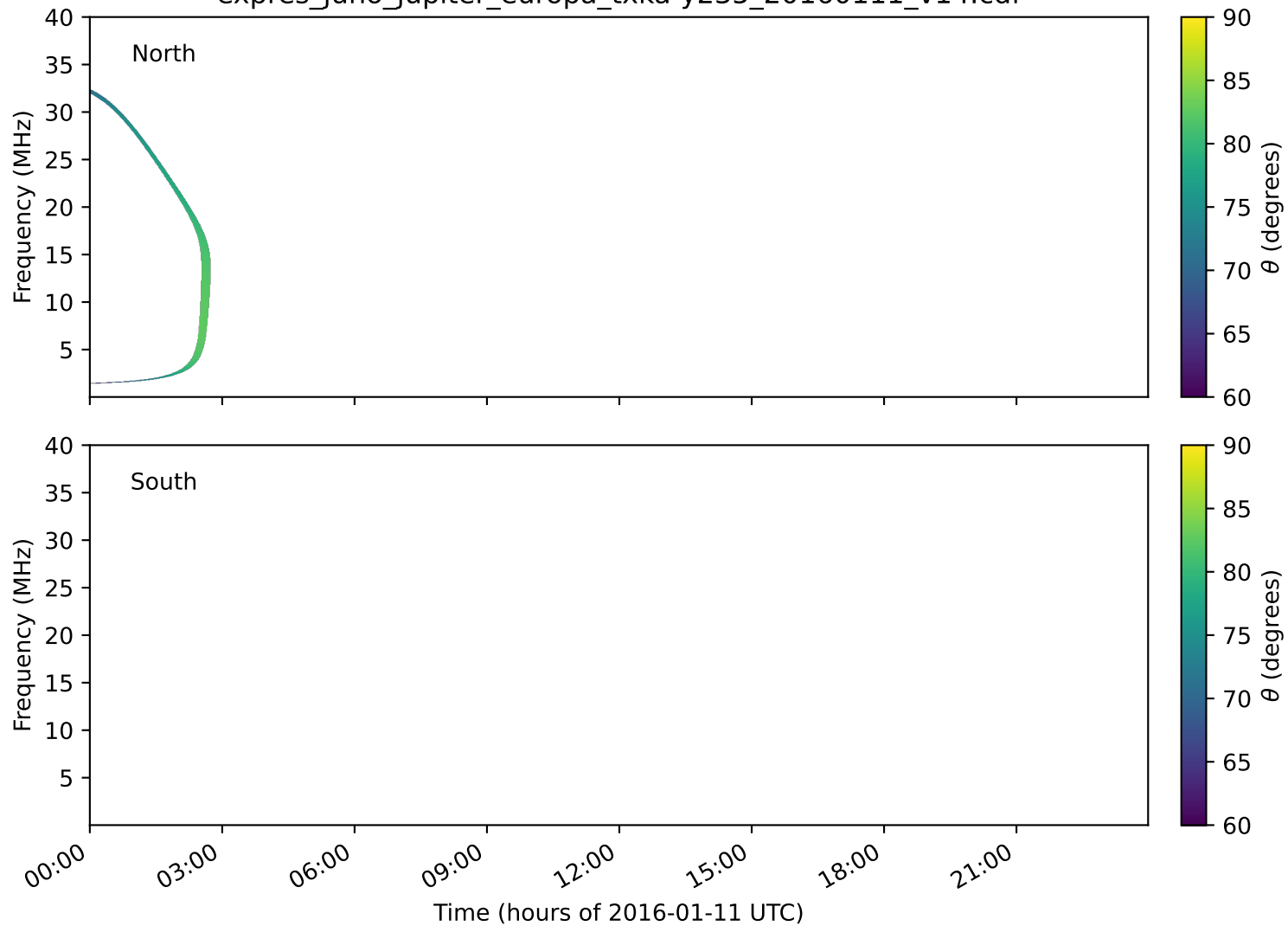
expres_juno_jupiter_europa_txka-y235_20160111_v14.cdf
