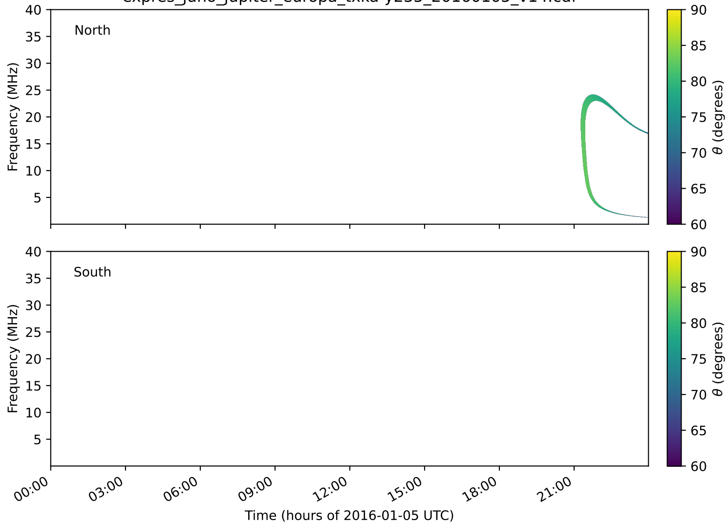
expres_juno_jupiter_europa_txka-y235_20160105_v14.cdf
