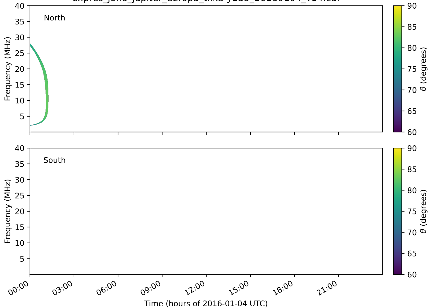
expres_juno_jupiter_europa_txka-y235_20160104_v14.cdf
