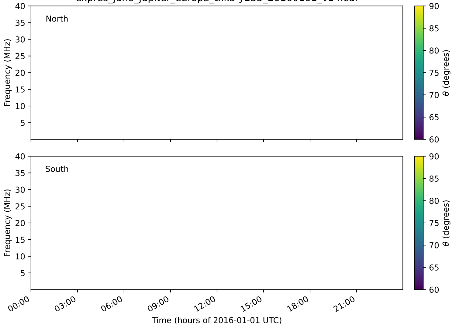
expres_juno_jupiter_europa_txka-y235_20160101_v14.cdf
