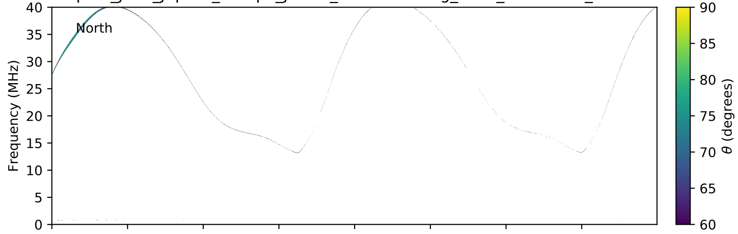
expres_juno_jupiter_europa_jrm09_lossc-wid1deg_3kev_20160131_v01.cdf
