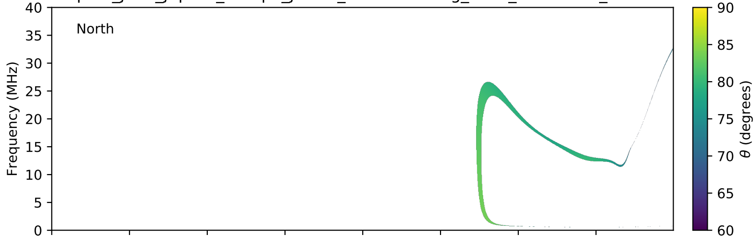
expres_juno_jupiter_europa_jrm09_lossc-wid1deg_3kev_20160123_v01.cdf
