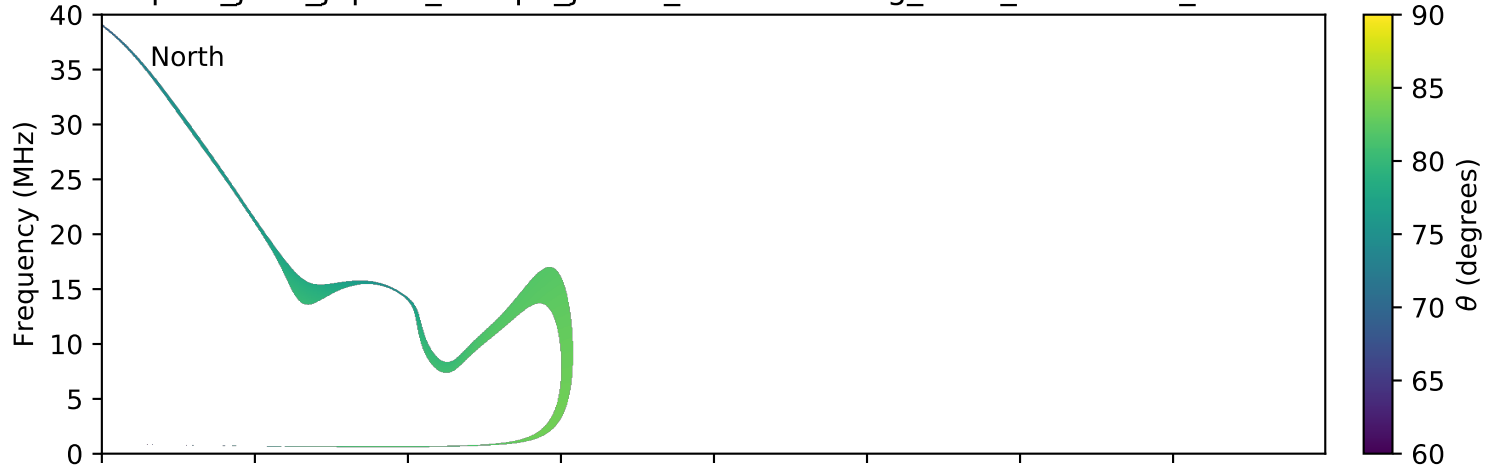
expres_juno_jupiter_europa_jrm09_lossc-wid1deg_3kev_20160111_v01.cdf
