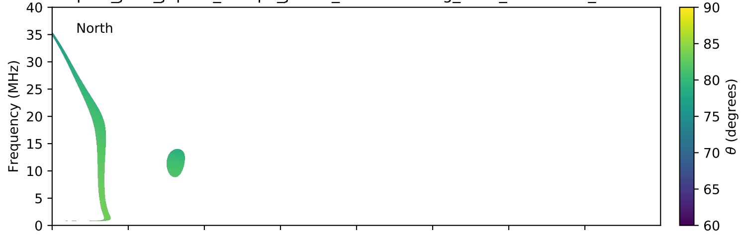
expres_juno_jupiter_europa_jrm09_lossc-wid1deg_3kev_20160104_v01.cdf
