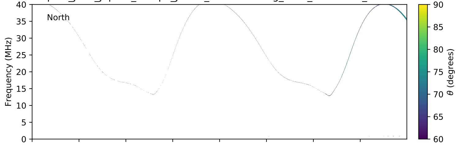
expres_juno_jupiter_europa_jrm09_lossc-wid1deg_3kev_20160103_v01.cdf
