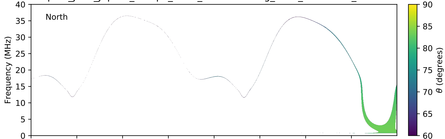
expres_juno_jupiter_europa_isaac_lossc-wid1deg_3kev_20160128_v01.cdf
