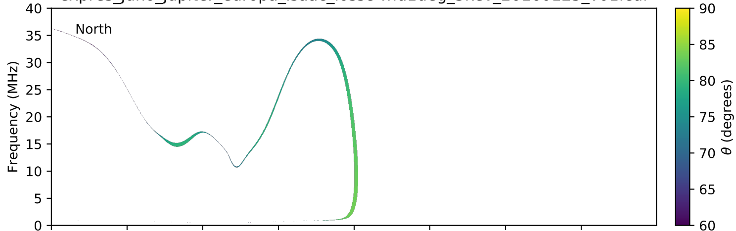
expres_juno_jupiter_europa_isaac_lossc-wid1deg_3kev_20160125_v01.cdf
