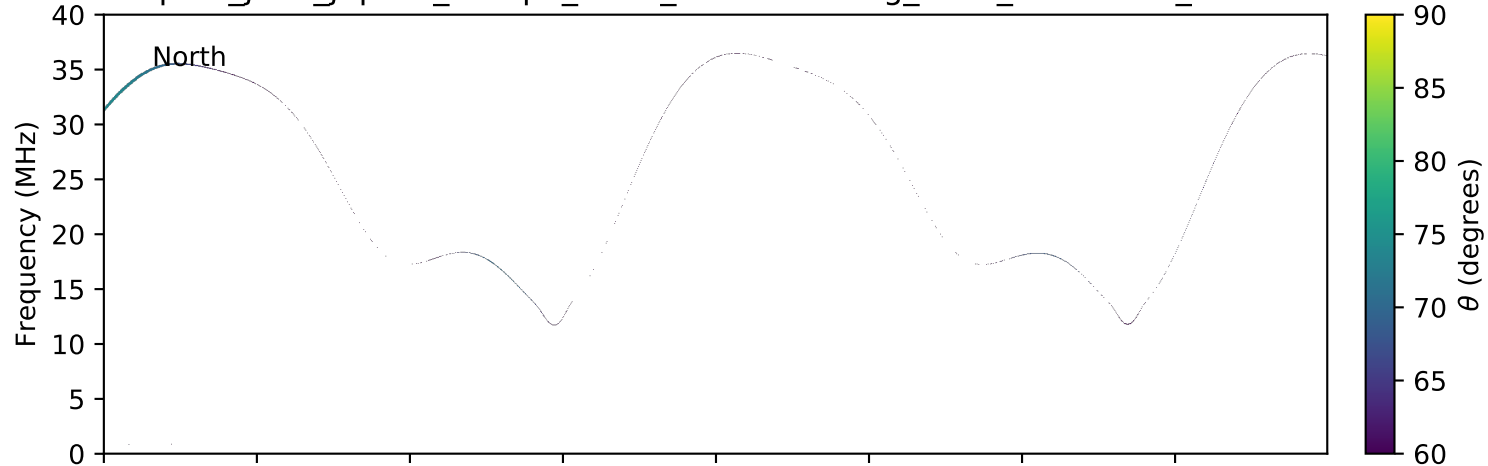
expres_juno_jupiter_europa_isaac_lossc-wid1deg_3kev_20160124_v01.cdf
