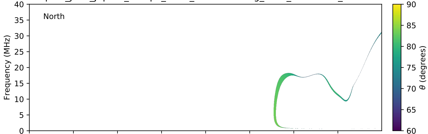
expres_juno_jupiter_europa_isaac_lossc-wid1deg_3kev_20160123_v01.cdf
