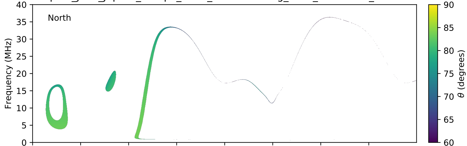
expres_juno_jupiter_europa_isaac_lossc-wid1deg_3kev_20160120_v01.cdf
