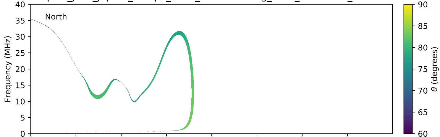
expres_juno_jupiter_europa_isaac_lossc-wid1deg_3kev_20160118_v01.cdf
