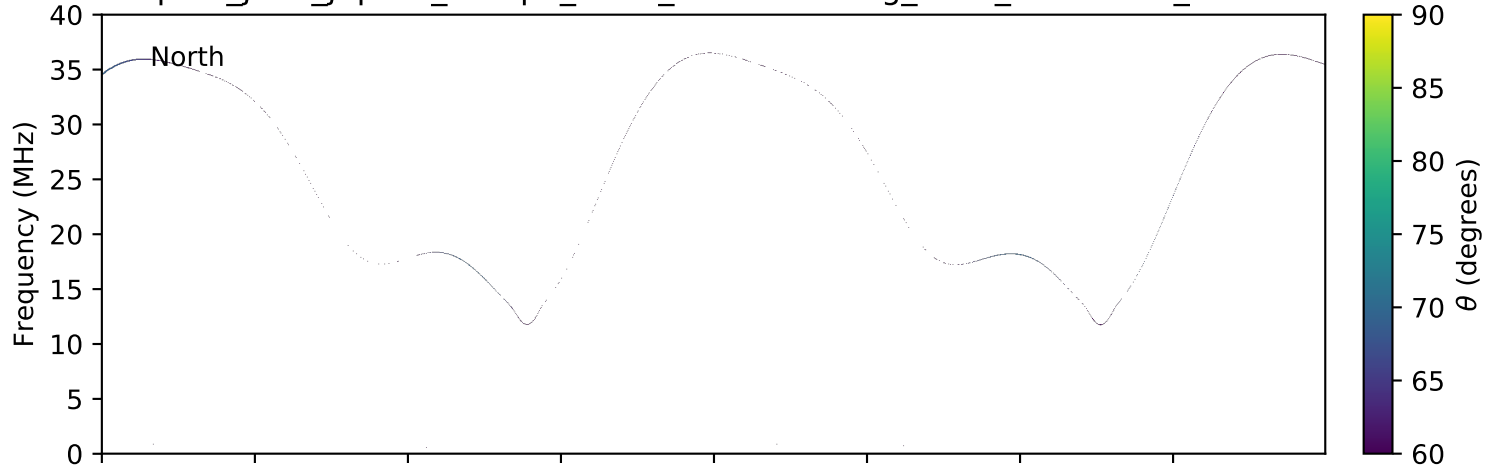
expres_juno_jupiter_europa_isaac_lossc-wid1deg_3kev_20160117_v01.cdf
