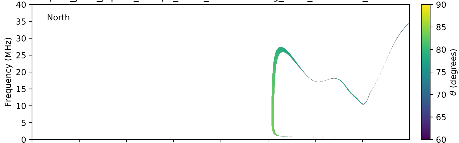
expres_juno_jupiter_europa_isaac_lossc-wid1deg_3kev_20160116_v01.cdf
