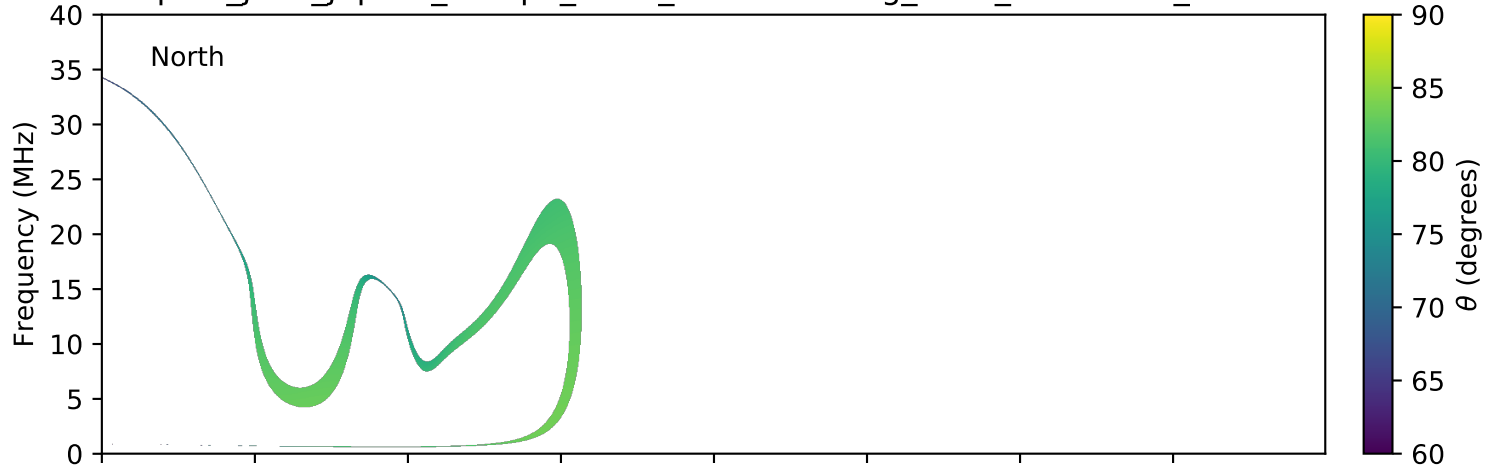
expres_juno_jupiter_europa_isaac_lossc-wid1deg_3kev_20160111_v01.cdf
