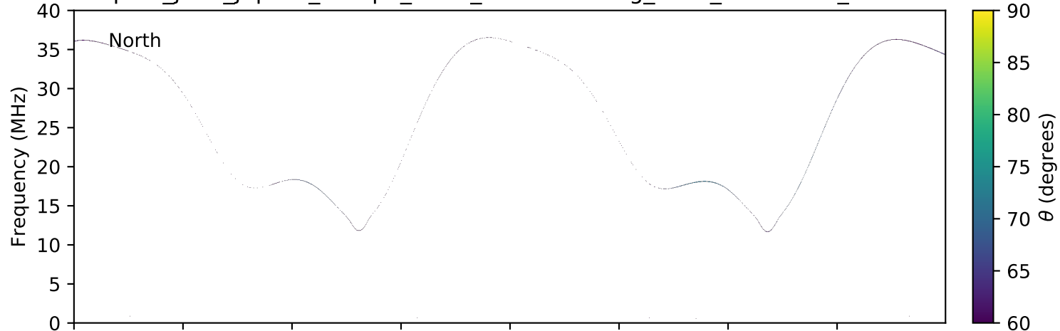
expres_juno_jupiter_europa_isaac_lossc-wid1deg_3kev_20160110_v01.cdf
