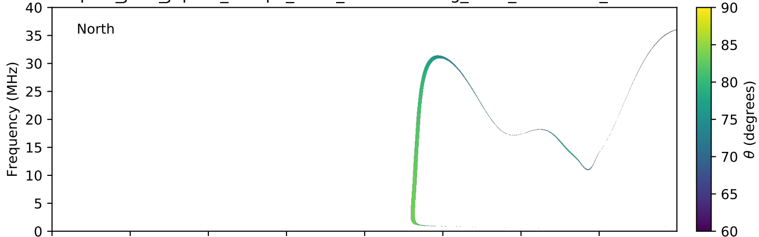
expres_juno_jupiter_europa_isaac_lossc-wid1deg_3kev_20160109_v01.cdf
