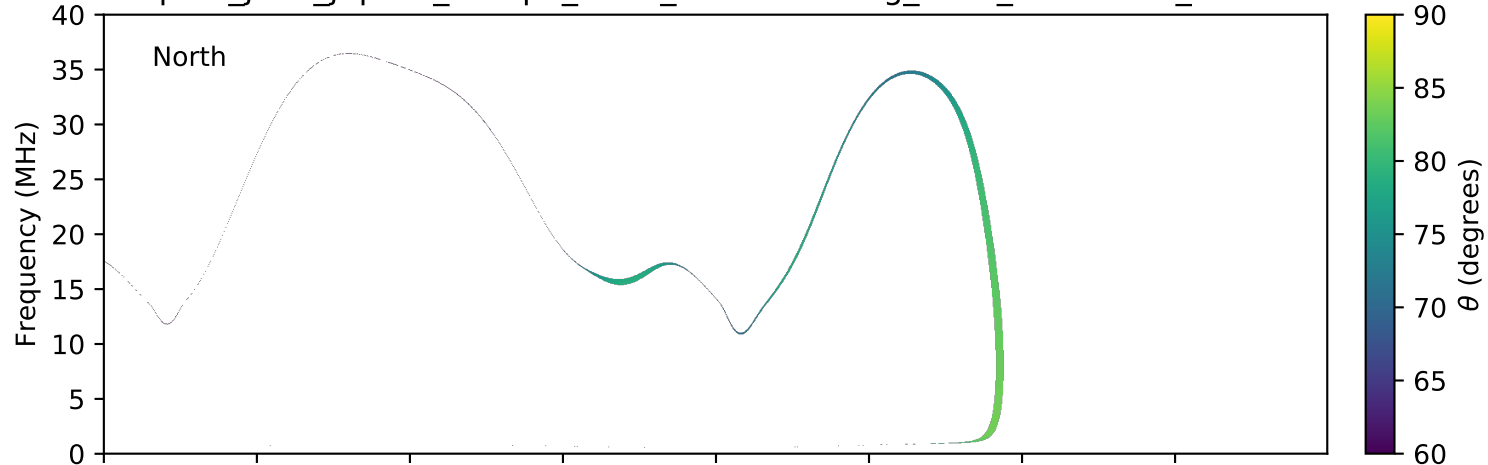
expres_juno_jupiter_europa_isaac_lossc-wid1deg_3kev_20160107_v01.cdf
